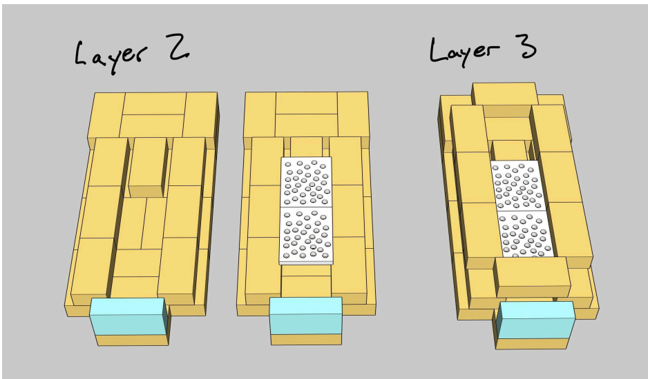
CDFE Extended Grate Layout
